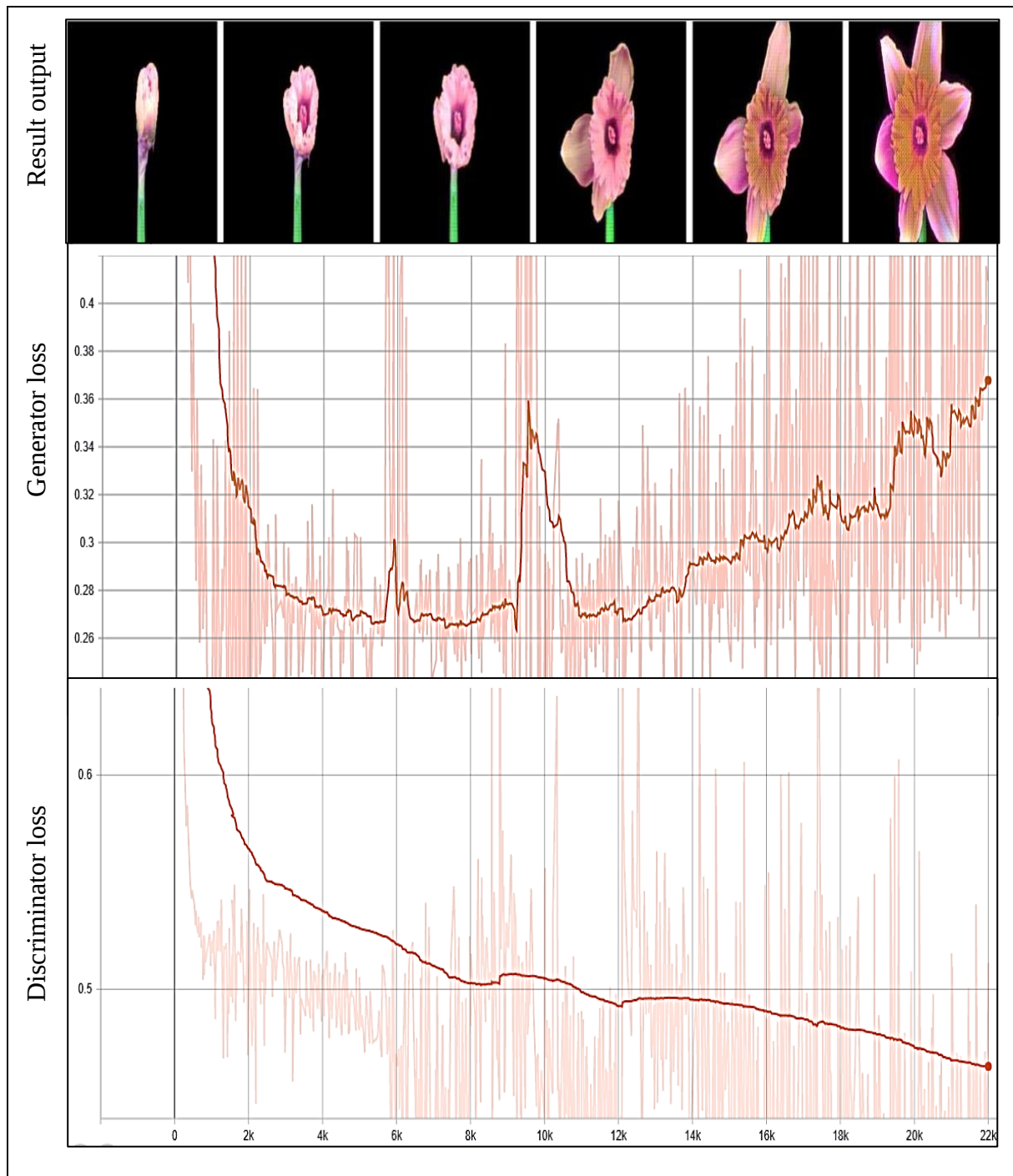
Figure 6-4 CC+CP+TD with gradient penalty
