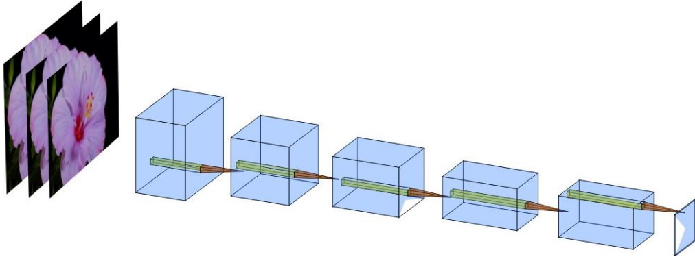
Figure 4-2 Temporal Discriminator Network
