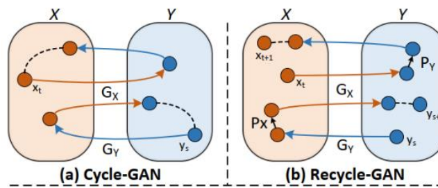
Figure 1-2 Cycle Gan vs Recycle GAN
