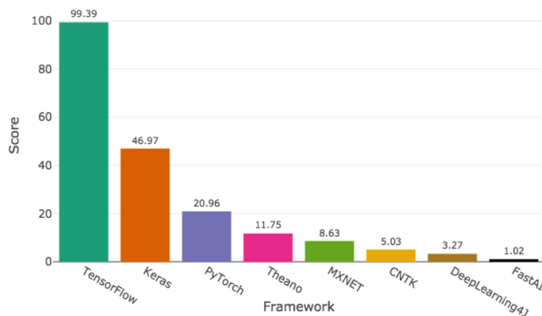
Figure 3-1 Deep Learning Framework comparison.
