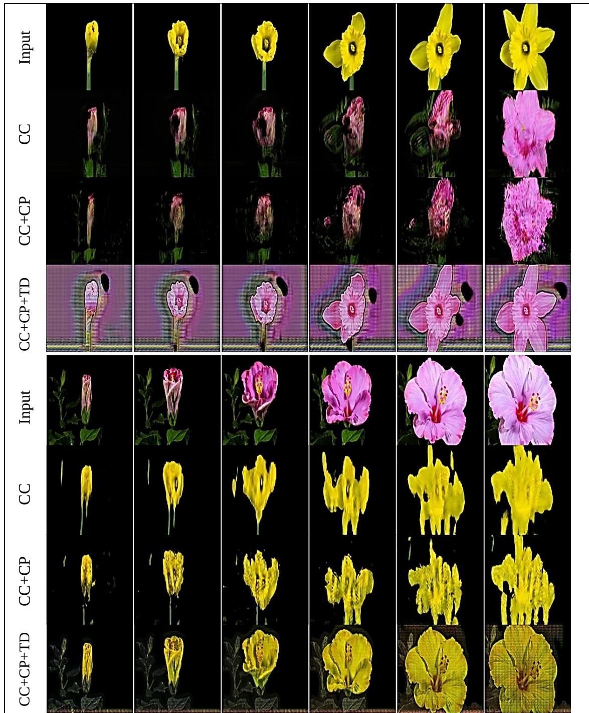
Figure 6-3 Flower to flower translation result
