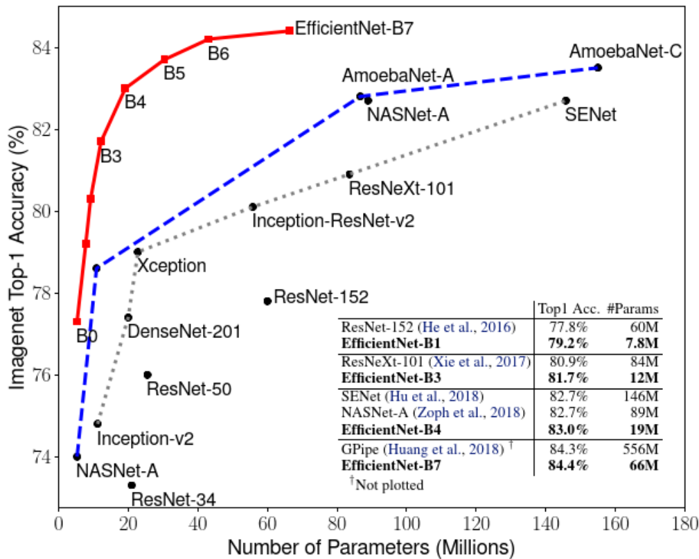
Figure 3-2 Benchmark Analysis on EfficientNet-B7
