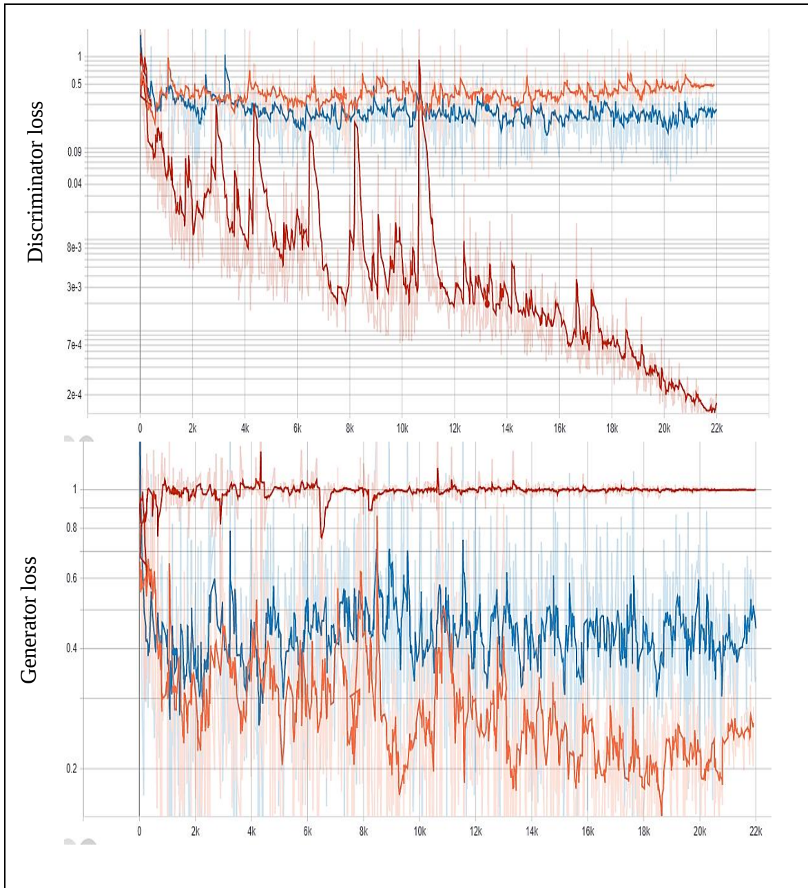
Figure 6-2 Training loss, vanishing problem on CC+CP+TD
