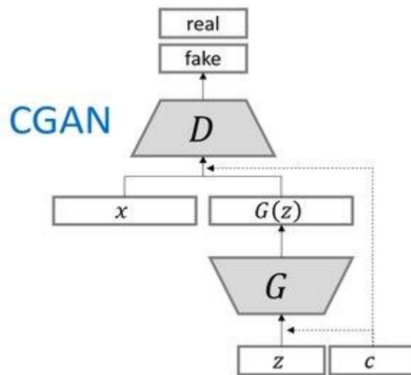
Figure 2-2 Conditional GAN Architecture
