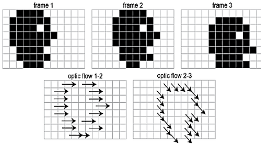
Figure 2-5 Detection of the optical flow in three consecutive images.
