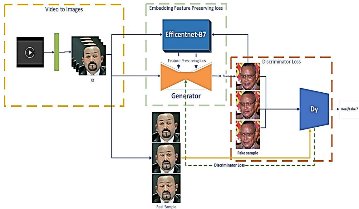
Figure 4-1 Model Architecture.
